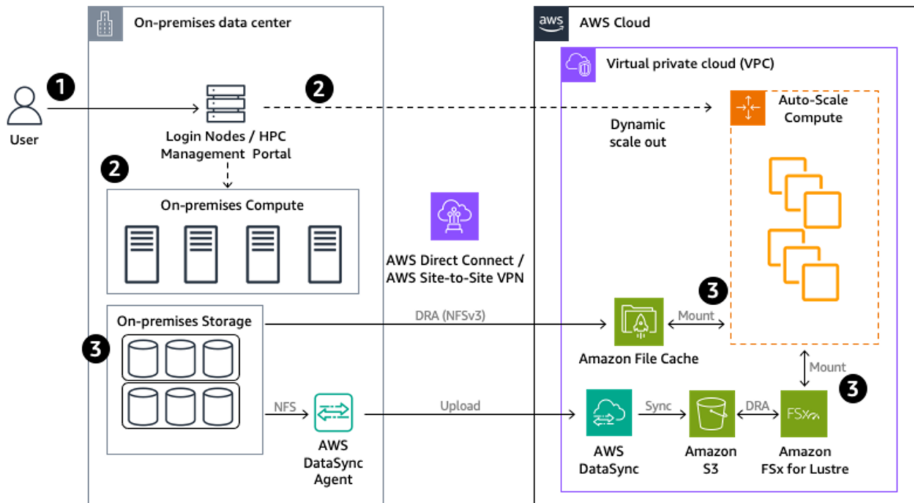
Reference architecture: Hybrid deployment
