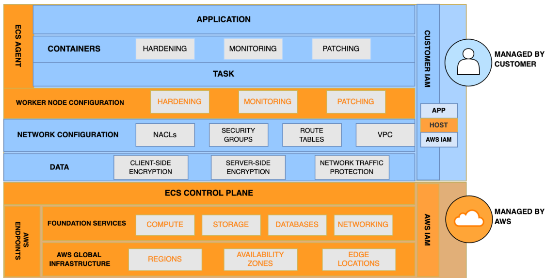
AWS Shared Responsibility Model for Amazon ECS with Fargate
